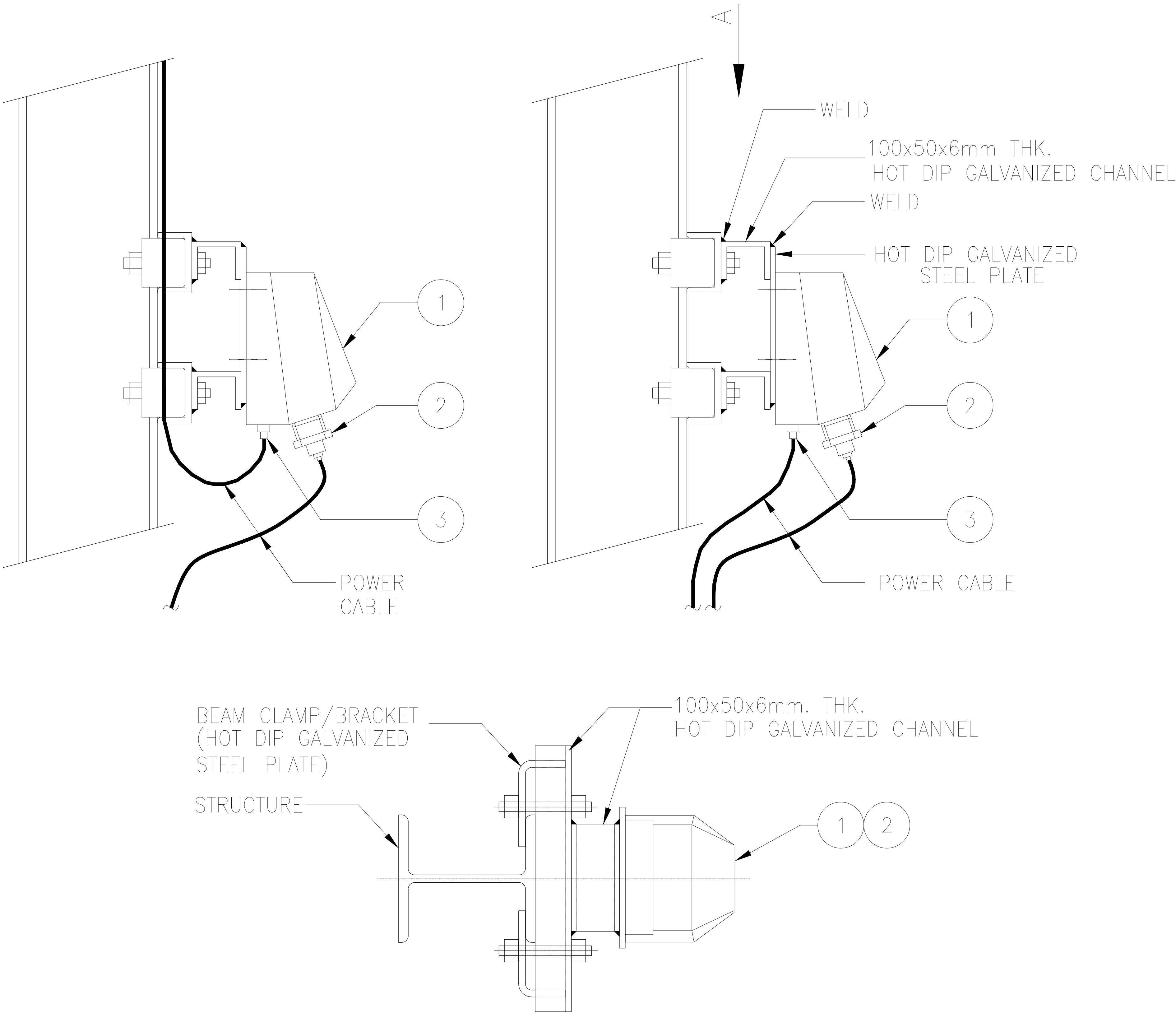
A VIEW
