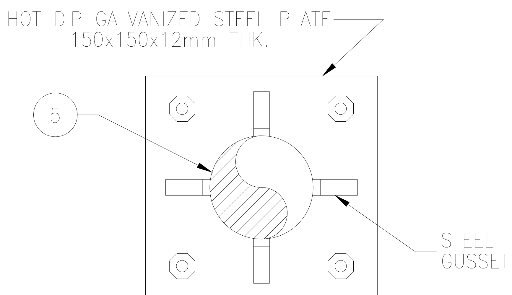
PLAN VIEW – BASE PLATE.
