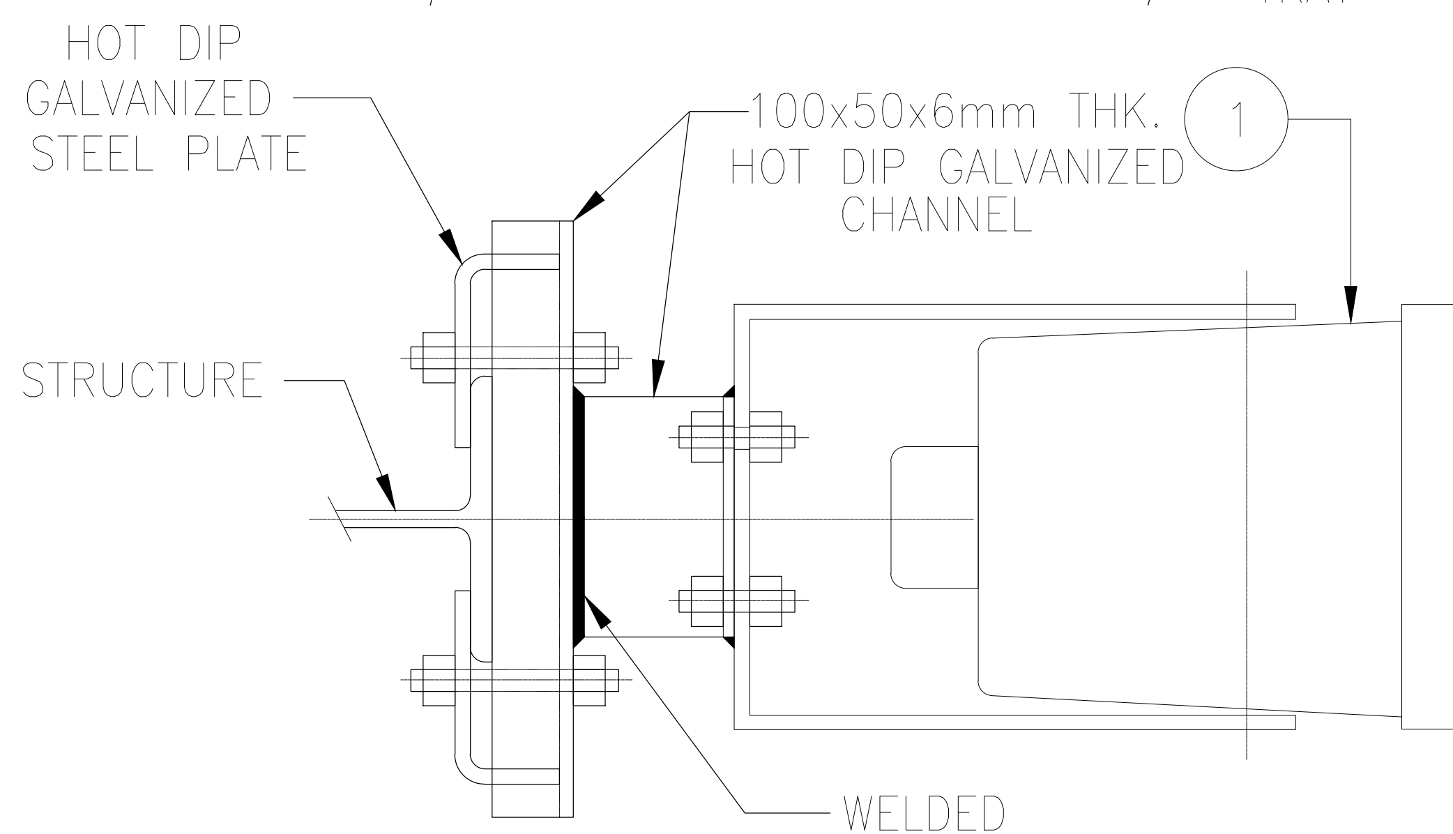
DETAIL 'A'
